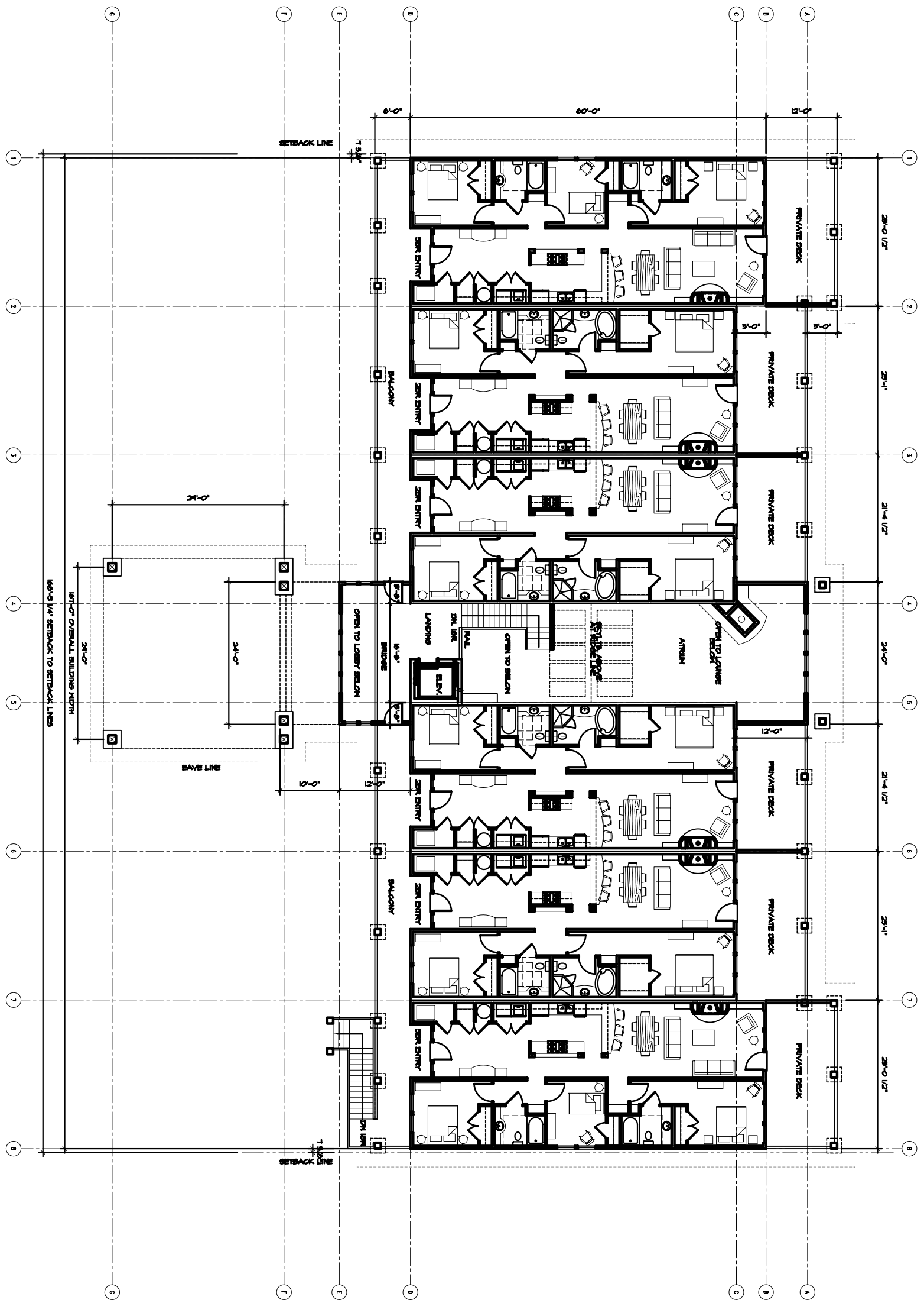
BUILDING UPPER FLOOR PLAN SCALE: 1/8" = 1'-0" 04/22/07
